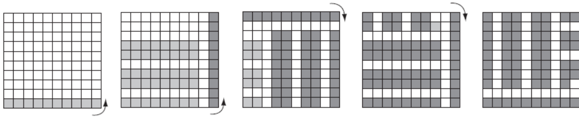
Figure 5: The Fill-and-Rotate algorithm applied to a 10 \times 10
