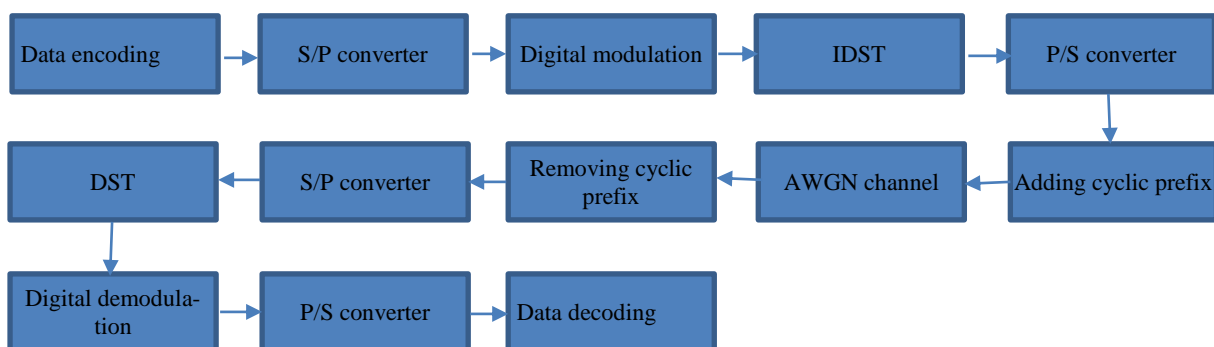
Figure 1. Block Diagram for Improved DST Based OFDM System
