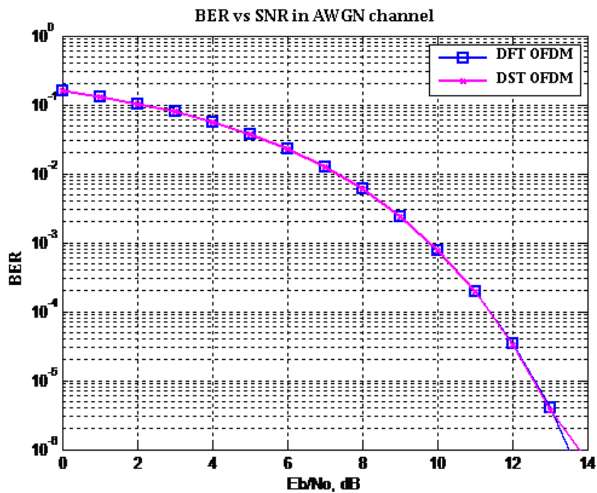
Figure 3. Performance of DST OFDM and DFT OFDM system under AWGN Channel with OOK modulation
