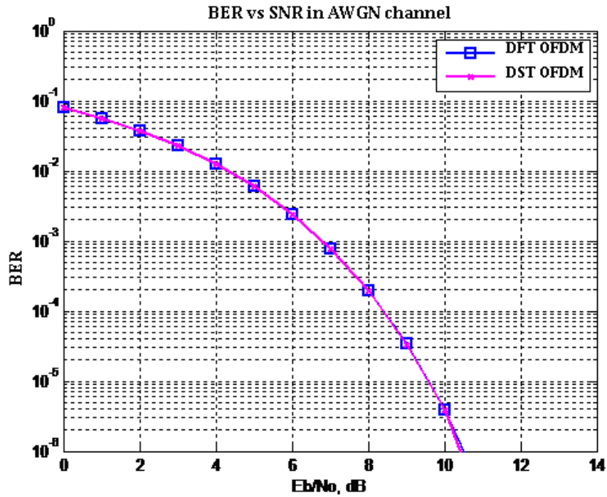
Figure 2. Performance of DST OFDM and DFT OFDM system under AWGN Channel with BPSK modulation
